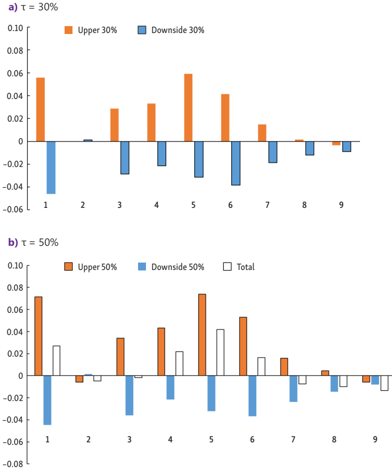
Figure 6. Information entropy
