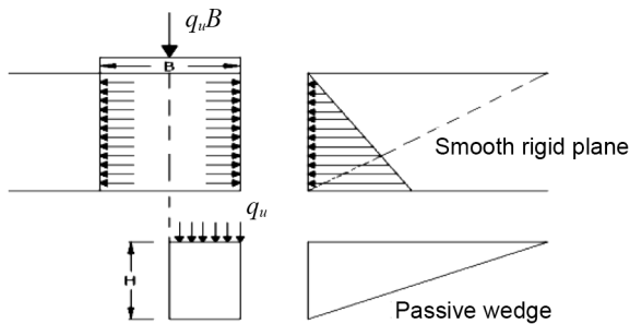
Fig. 3. Failure mechanism by Andrawes et al. (1996)
