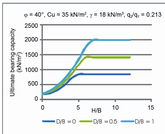
Fig. 6. Ultimate bearing capacity by Alkarni's equation
