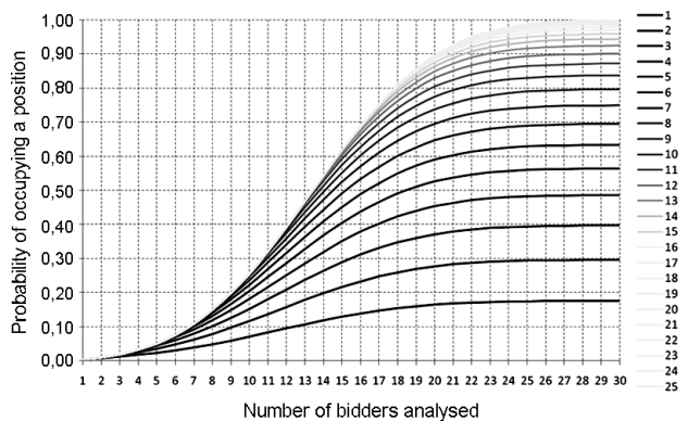
Fig. 2. Single bidder’s position performance calculation accuracy
