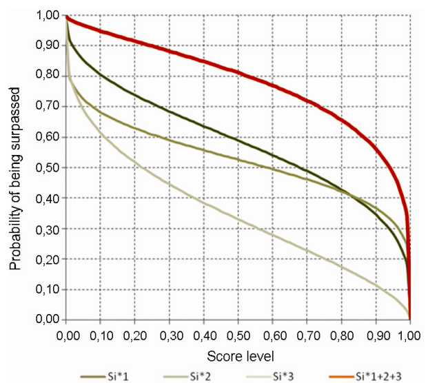
Fig. 4. Scoring performance for several bidders
